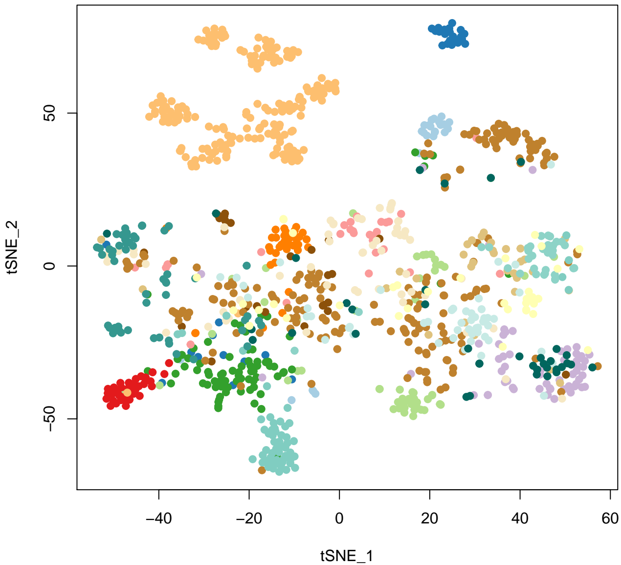
Z01, ReLU
